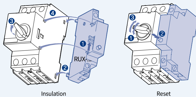
Insulation barrier
