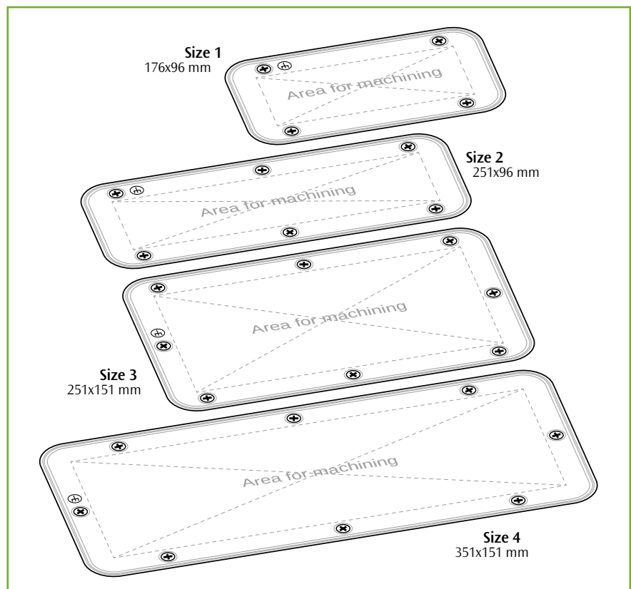
Conductive earth flange with single screw (identified with marking).
