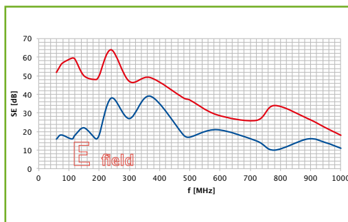
ST wall mounting boxes (EMC vs. standard)
