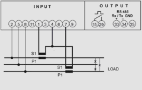
Three-phase 3Ph network, unbalanced load (aron L1-L3)
