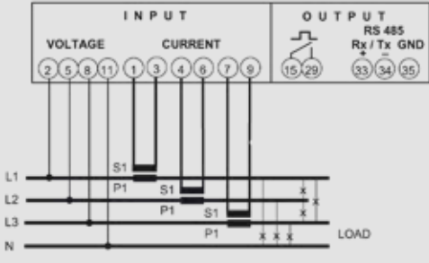
Three-phase 3Ph +N network, unbalanced load
