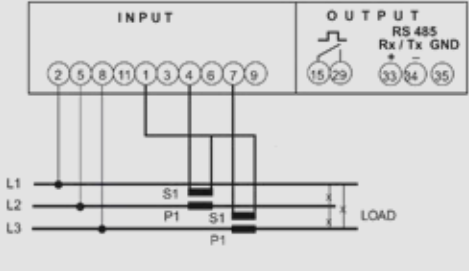
Three-phase 3Ph network, unbalanced load (aron L2-L3)
