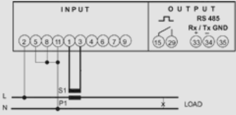
Single-phase network,
