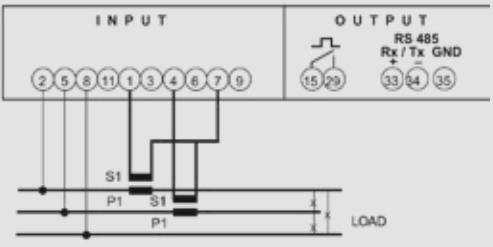
Three-phase 3Ph network, unbalanced load (aron L1-L2)
